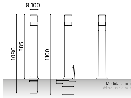
PFLEXHNL PFLEXHNL + BEXTRAP01 PFLEXHNPL
